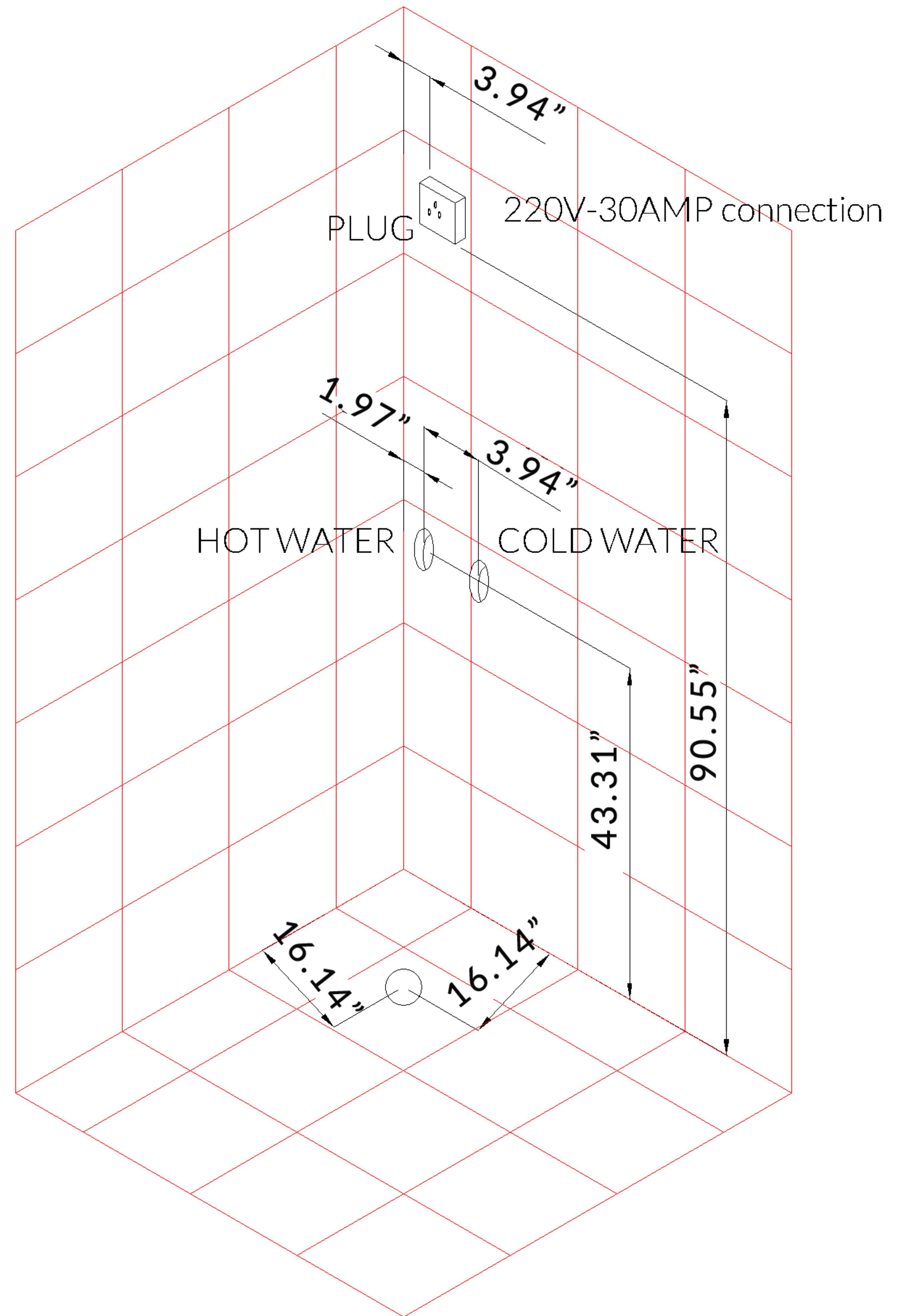
DZ961F8 INSTALLATION (RIGHT) DIMENSIONS: 59" x 35" x 89"
