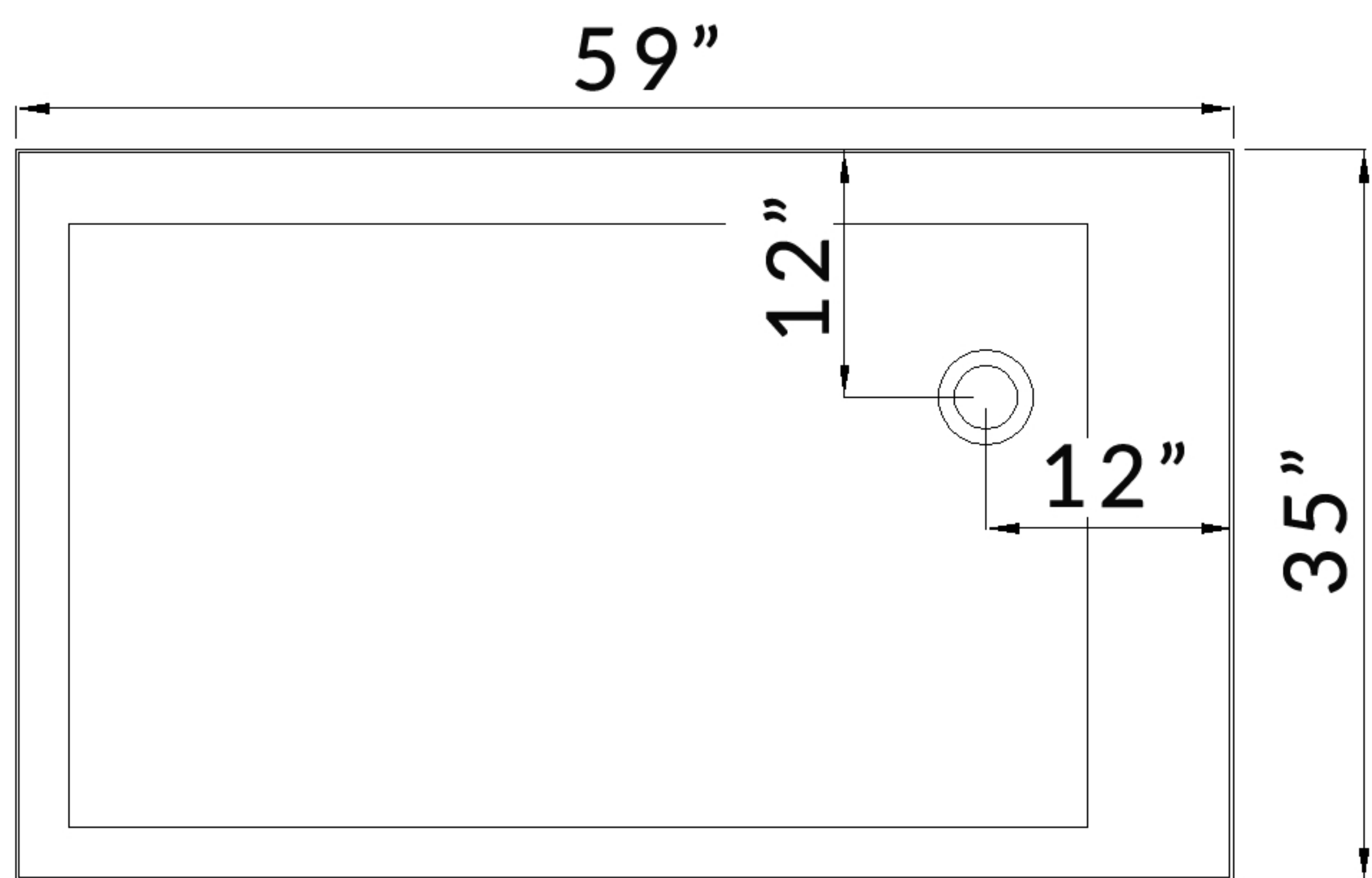
DZ961F8 INSTALLATION (RIGHT) DIMENSIONS: 59" x 35" x 89"
